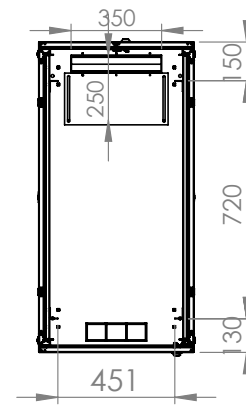
Detail View
